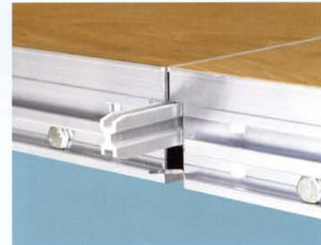
Added safety by the X-junction part
