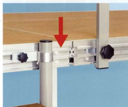
Clever – continuous assembly rail
